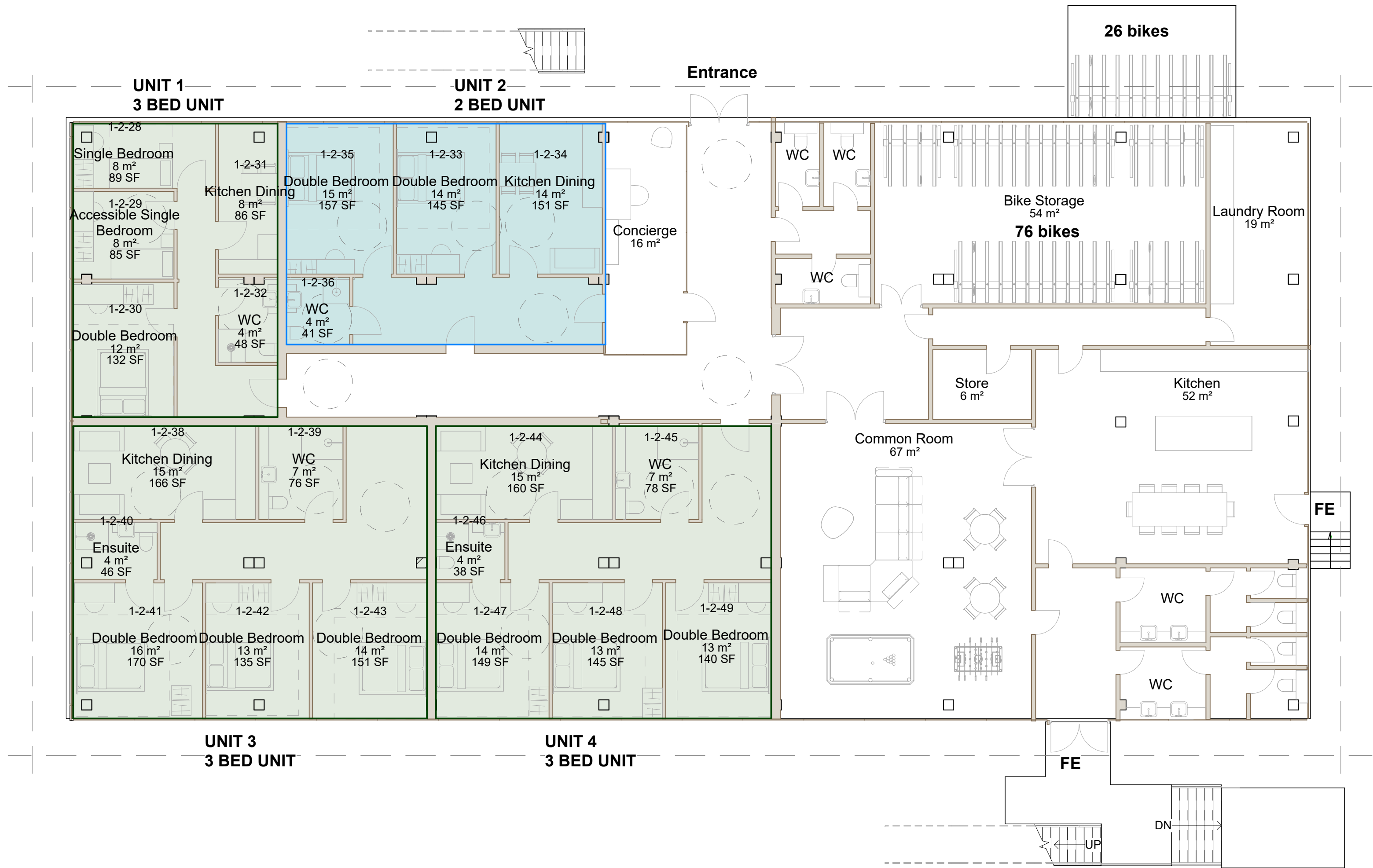
1 Proposed 00. Ground floor 1 : 100
