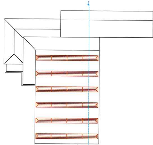
02 ROOF PLAN (1) 1:100
