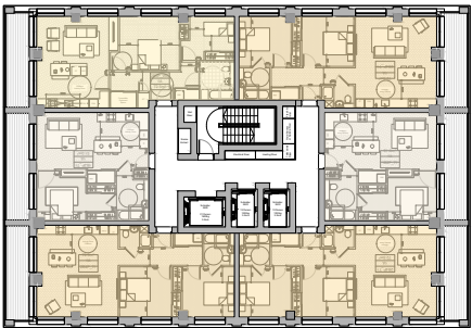
Tower 1A typical floor plan
